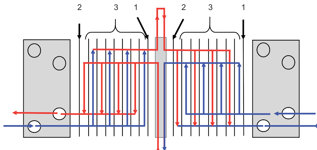
Figure 3 : Exemple de configuration multi-sections.
